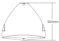
Dimensions(Unit: mm)
